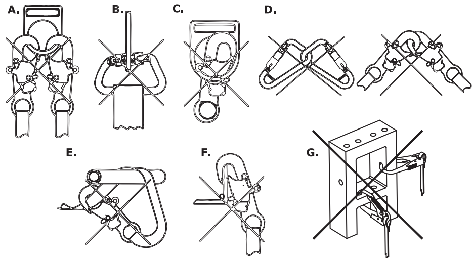
Figure 5 - Inappropriate Connections
